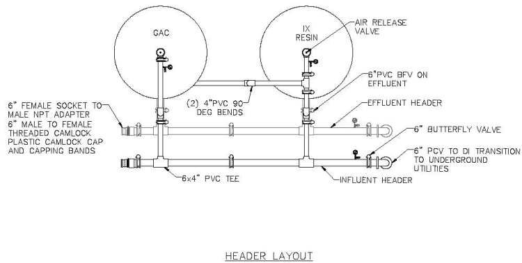
HEADER LAYOUT
